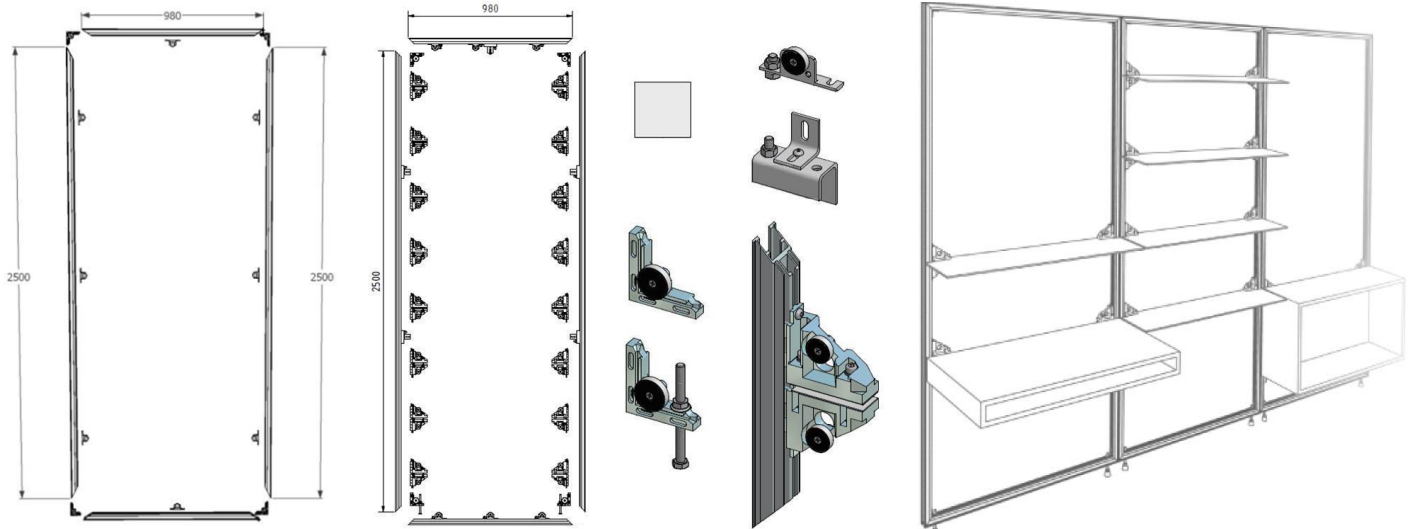
Frame components
