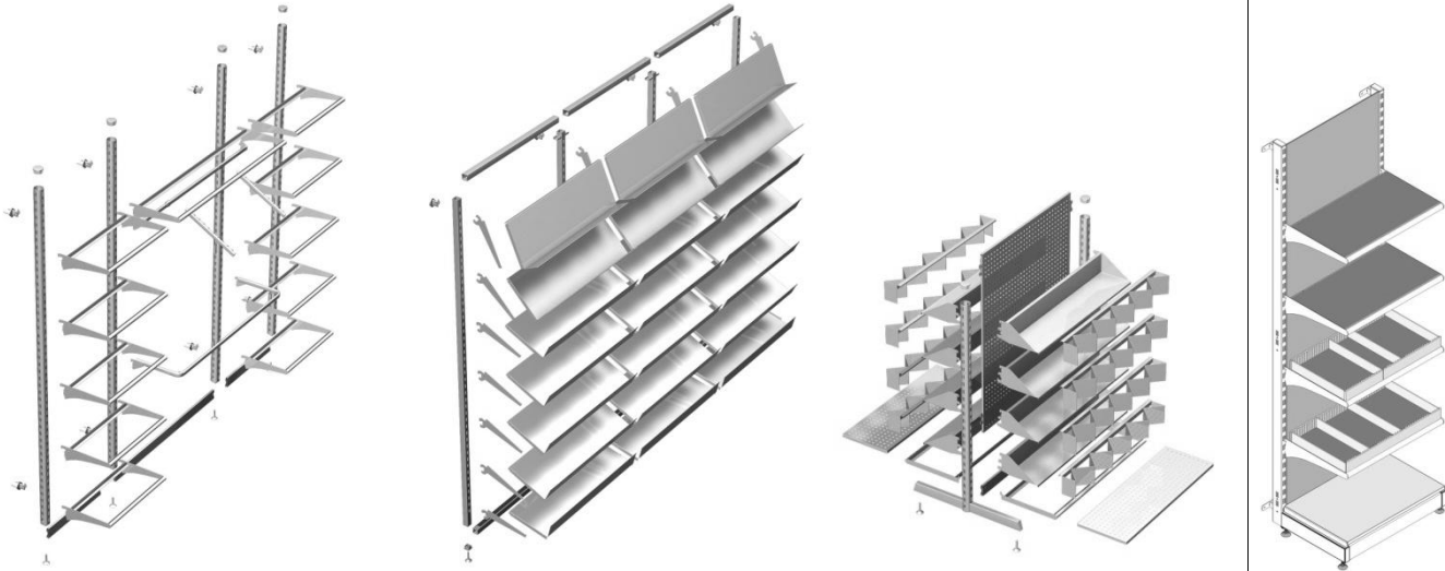
Frame components
